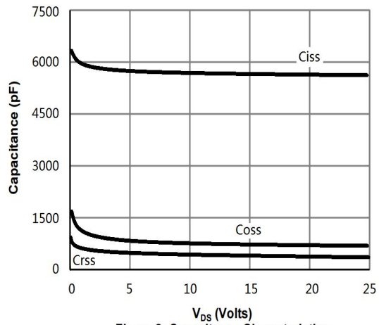
Figure 8: Capacitance Characteristics
