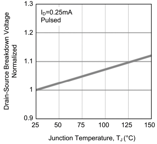
2. Breakdown Voltage vs. Junction Temperature
